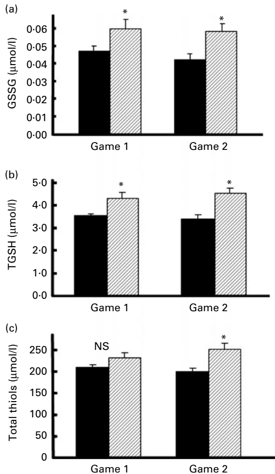
Fig. 1. (a–c) Pre-game (■) and immediate post-game (▨) values for GSSG, total glutathione (TGSH) and total thiols following two soccer games separated by 72 h in elite female players ( n 16). *Mean values were significantly higher than the pre-game values ( P < 0.05 ).
