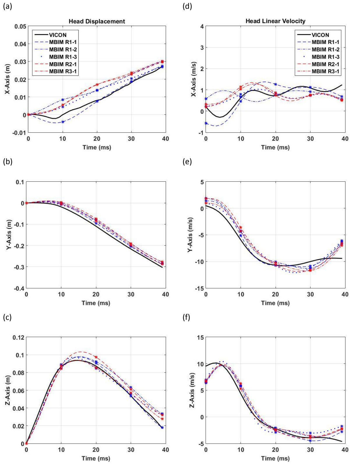
Figure 6: Head CG displacement (a-c) and linear velocity (d-f) in the global coordinate system (Figure 4) calculated with the reflective marker-based motion analysis (Black line) and the model-based image-matching technique for Researcher 1 (R1) (Blue lines) and Researcher 2 (R2) and 3 (R3) (Red lines). The MBIM discrete measures are indicated with markers.
