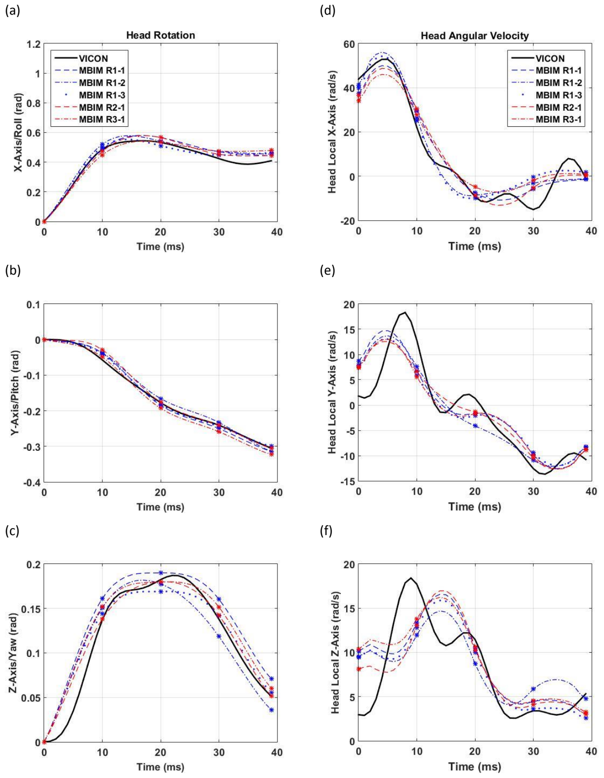
Figure 7: Head CG rotation for Roll (X), Pitch (Y) and Yaw (Z) angles (a-c) and the head angular velocity about the local head axes (d-f), see Figure 3, calculated with the reflective marker-based motion analysis (Black line) and the model-based image-matching technique for Researcher 1 (R1) (Blue lines) and Researcher 2 (R2) and 3 (R3) (Red lines). The MBIM discrete measures are indicated with markers.
