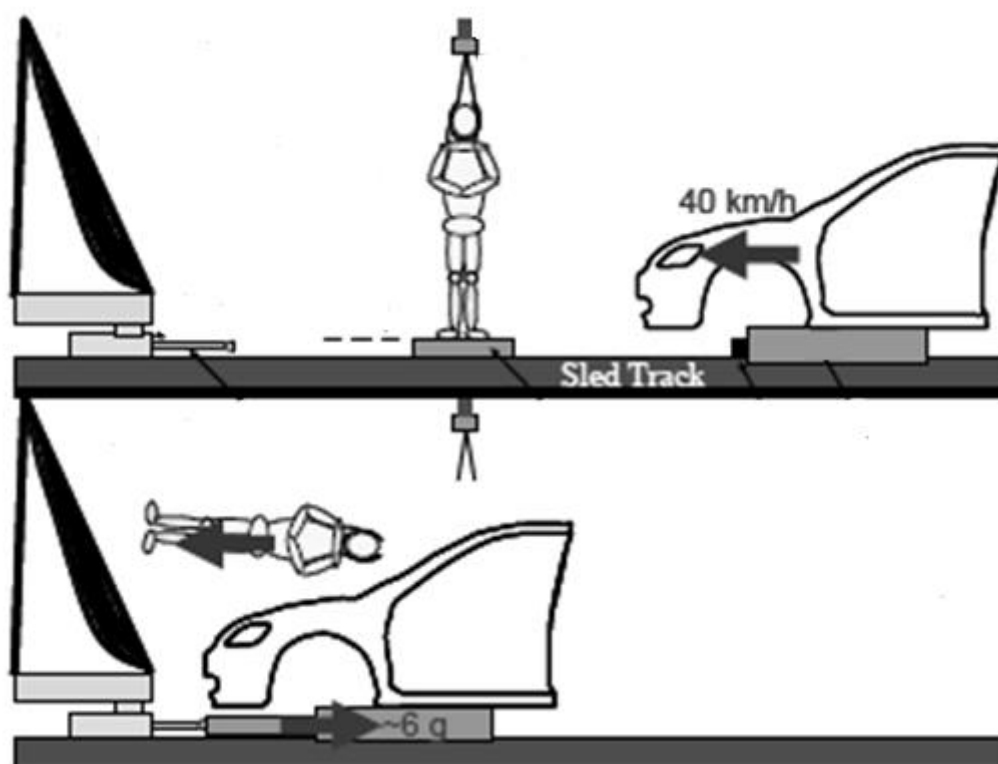
Figure 1: Schematic of the Vehicle-cadaver impact
