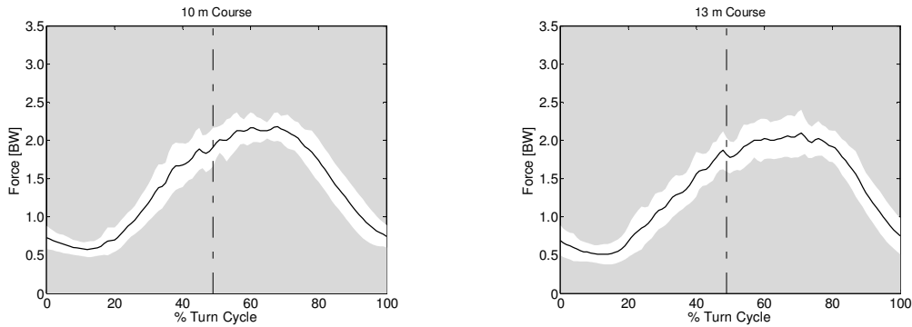
Figure 9.39: The ensemble average of reaction force-time relation in the 10 meter (left) and the 13 (right) meter courses, \pm SD (white area), SID 10.
