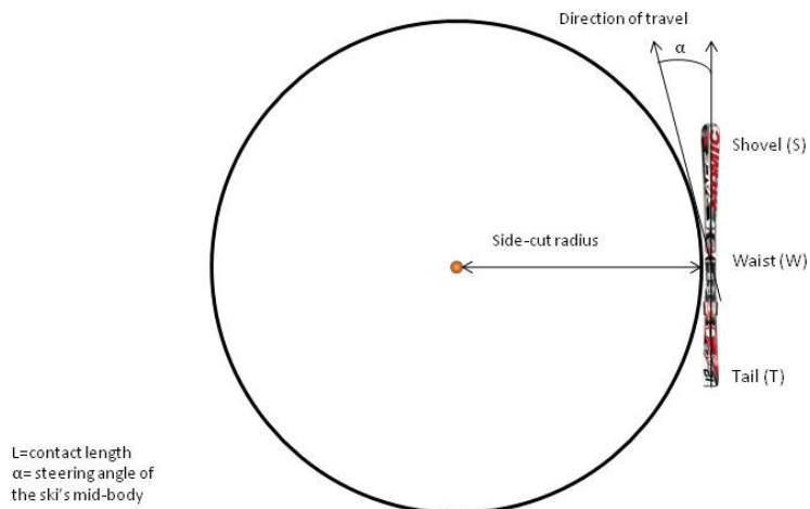
Figure 2.1: The side-cut radius and the steering angle of a modern slalom ski.
