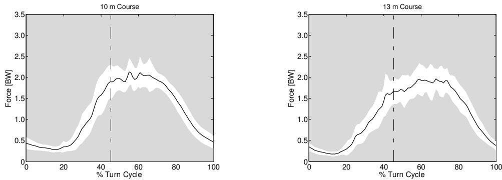
Figure 9.16: The ensemble average of reaction force-time relation in the 10 meter (left) and the 13 (right) meter courses, \pm SD (white area), SID 4.
