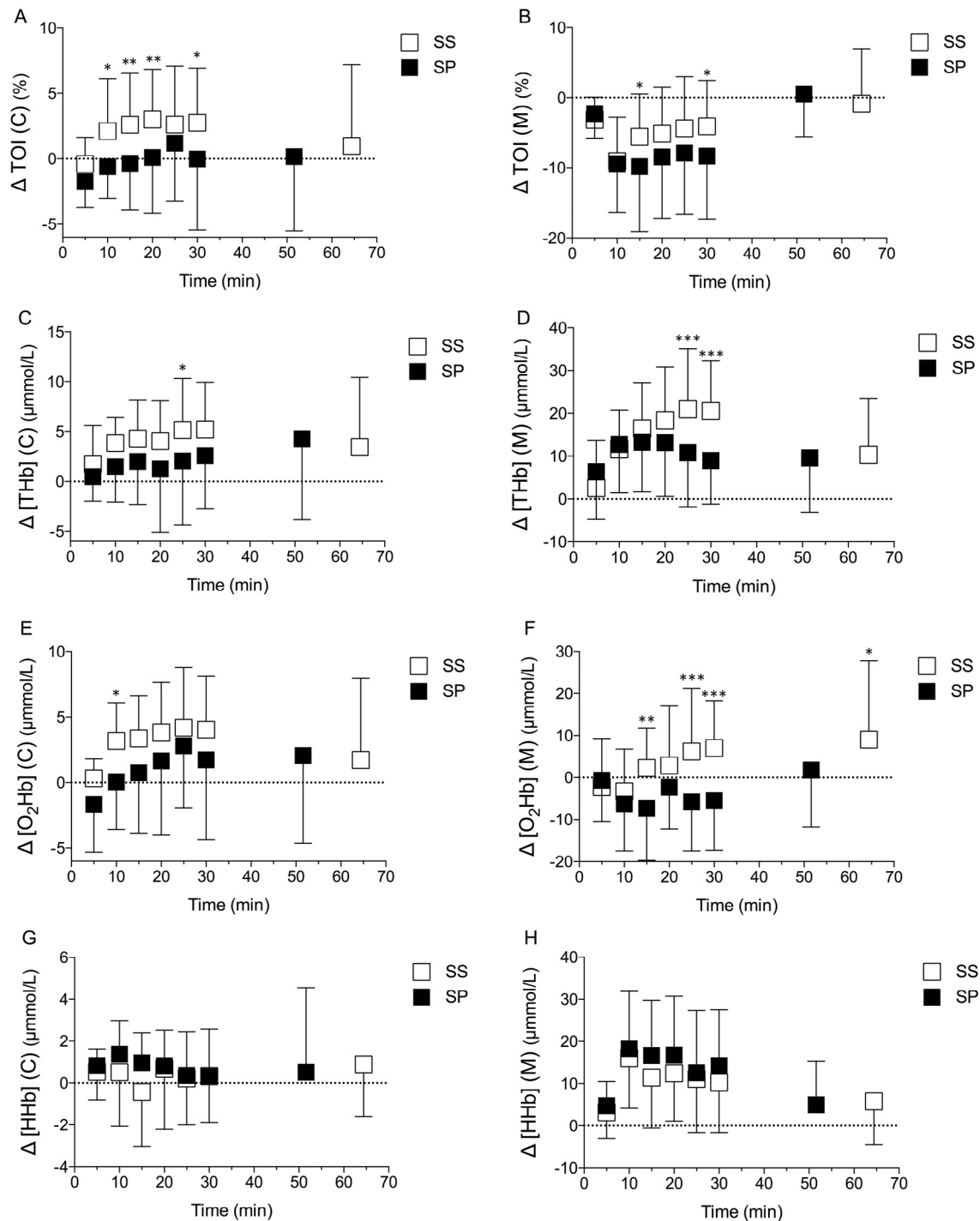
Fig. 4. Values of \Delta TOI (A, B), \Delta THb (C, D), \Delta O 2 Hb (E, F), and \Delta HHb (G, H) in the first 30 min of exercise and at TTE during SS and SP measured in the prefrontal cortex (C) and on vastus lateralis muscle (M) (mean \pm SD). * p < 0.05 , ** p < 0.01 , *** p < 0.001 , n = 12 . HHb = deoxyhemoglobin; O 2 Hb = oxyhemoglobin; SP = snus placebo; SS = Swedish snus; TOI = tissue oxygenation index; THb = total hemoglobin; TTE = time to exhaustion.
